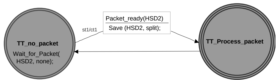
Figure 11-38. Transaction Translator
