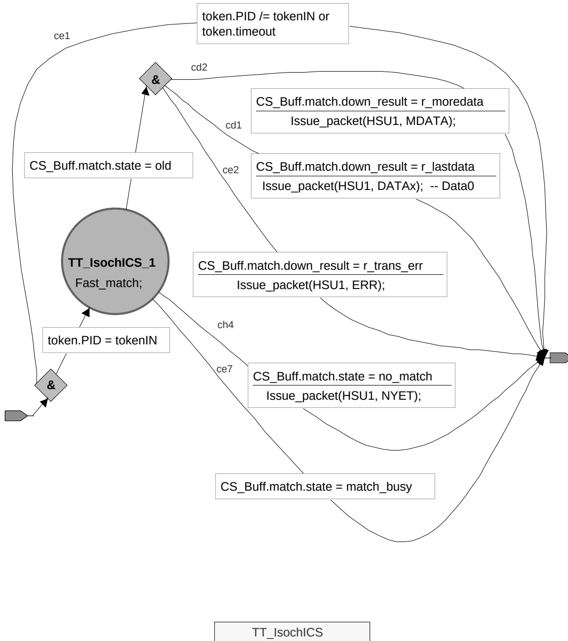
Figure 11-91. Isochronous IN Complete-split Transaction TT State Machine
