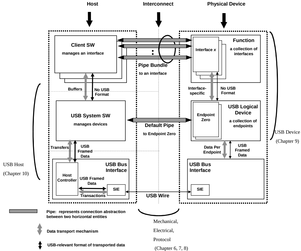
Figure 5-9. USB Host/Device Detailed View
