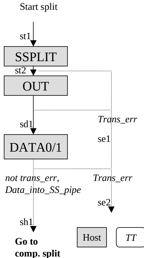
Figure 11-68. Interrupt OUT Start-split Transaction Sequence
