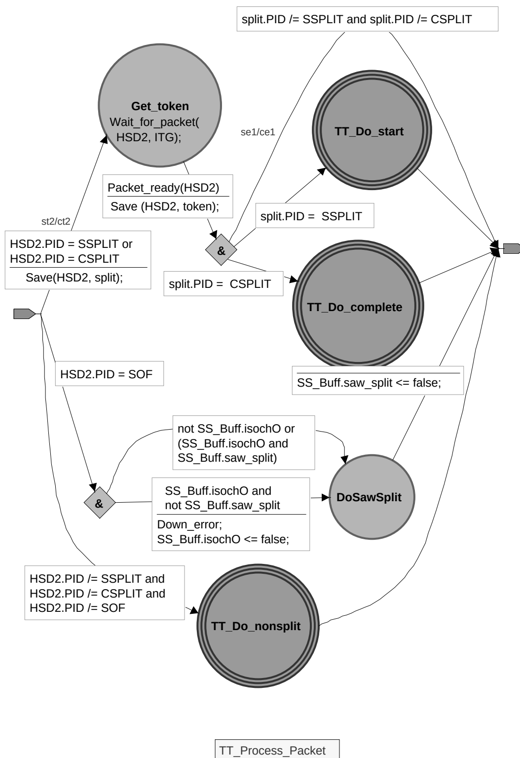
Figure 11-39. TT_Process_Packet
