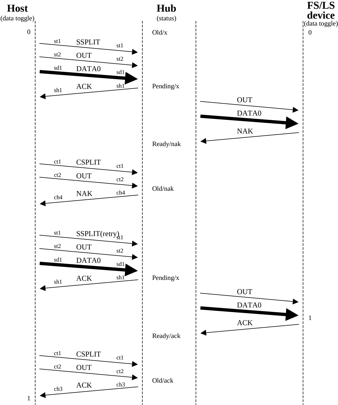
Figure A-22. Device Busy No Smash(FS/LS NAK)
