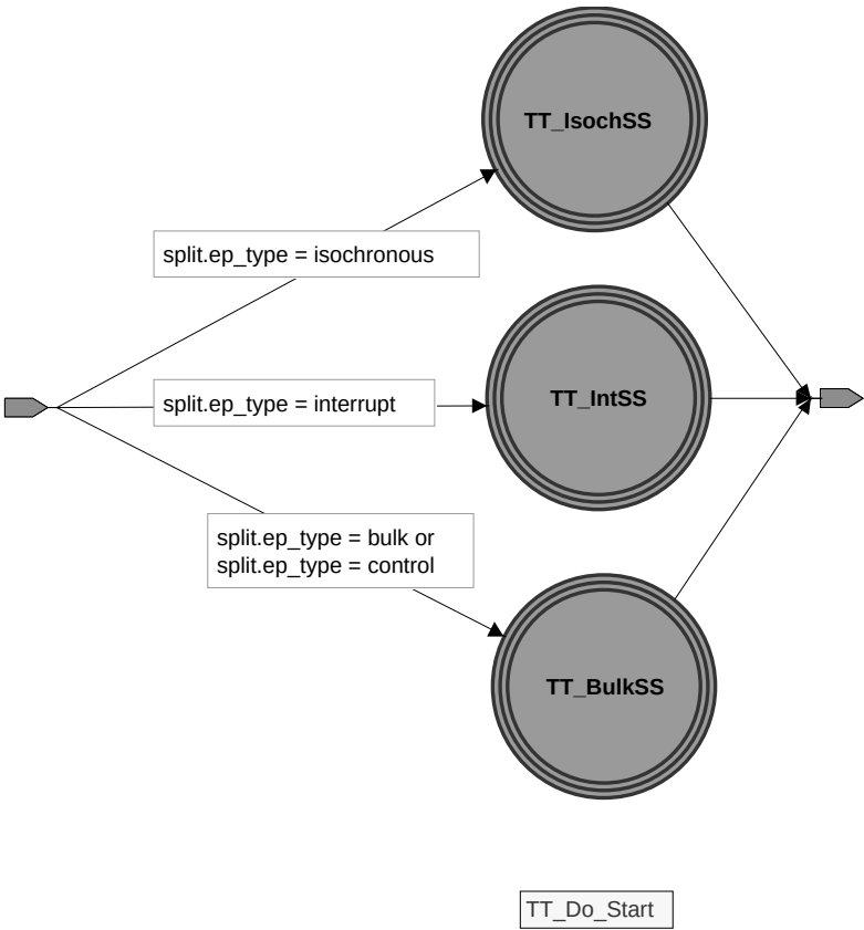
Figure 11-40. TT_Do_Start
