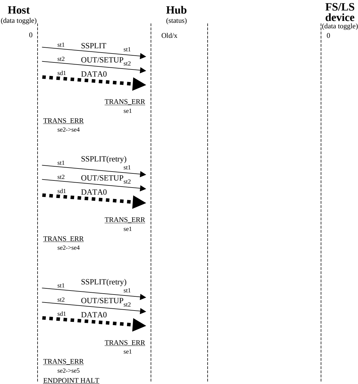
Figure A-3. Normal HS DATA0/1 3 Strikes Smash
