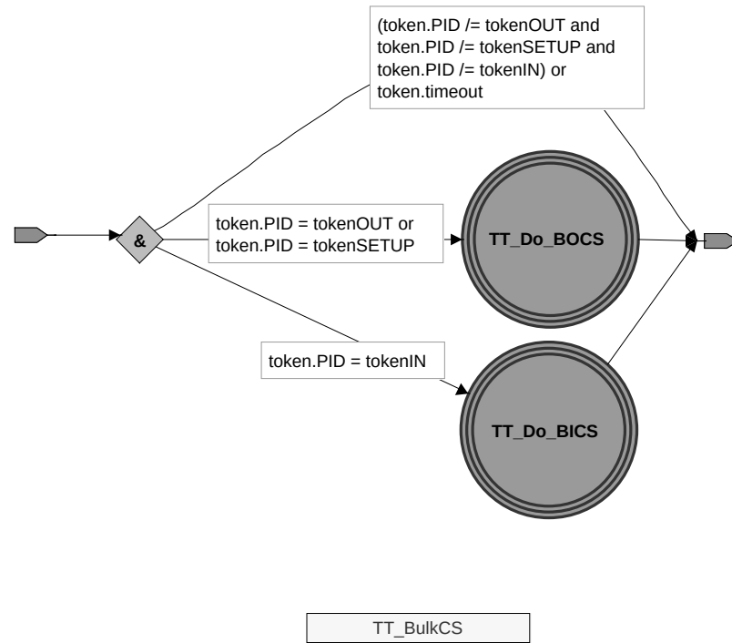
Figure 11-43. TT_BulkCS
