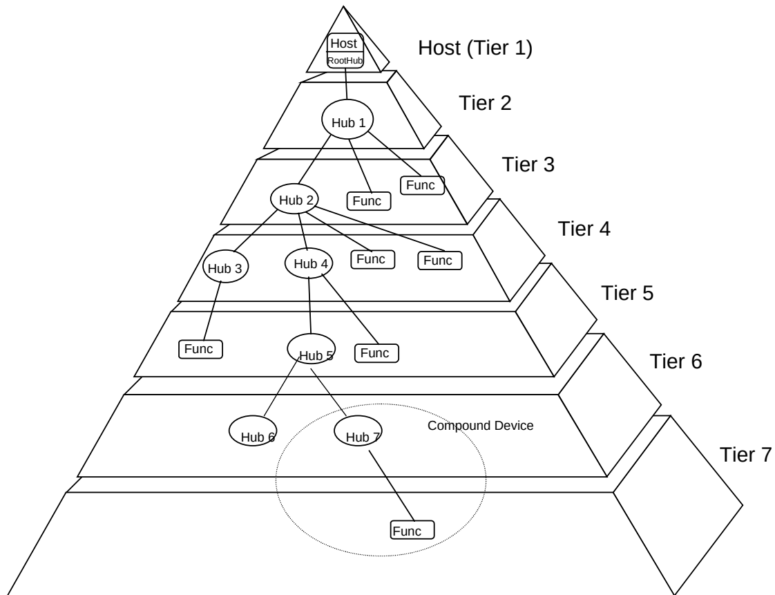
Figure 4-1. Bus Topology
