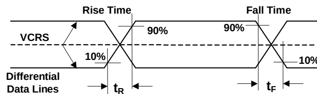
Figure 7-8. Data Signal Rise and Fall Time
