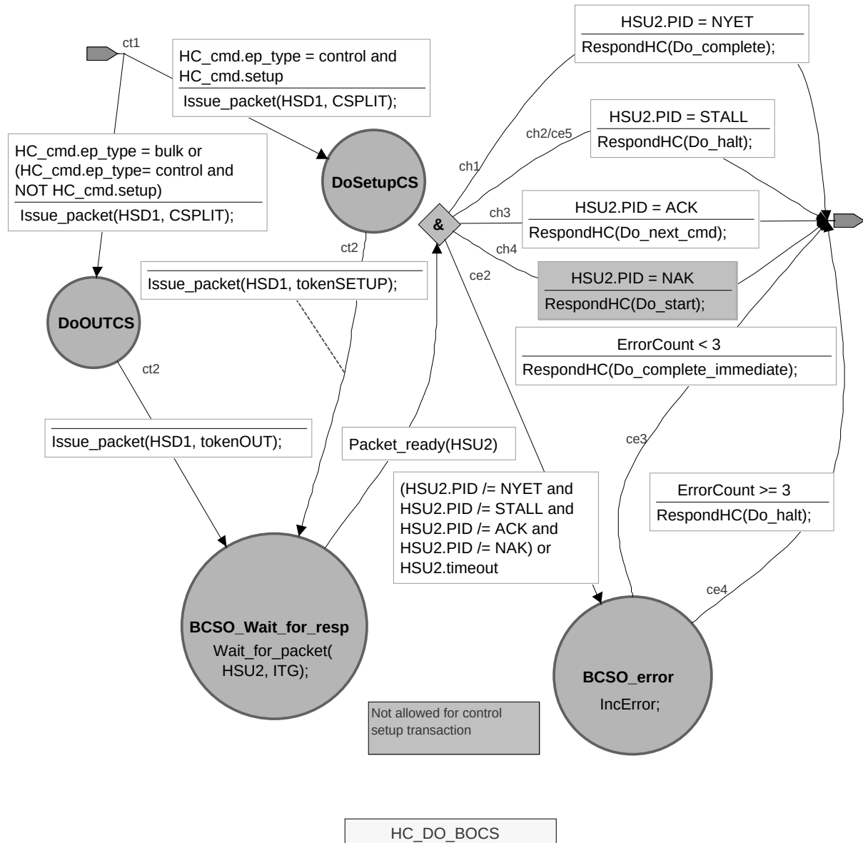
Figure 11-53. Bulk/Control OUT Complete-split Transaction Host State Machine
