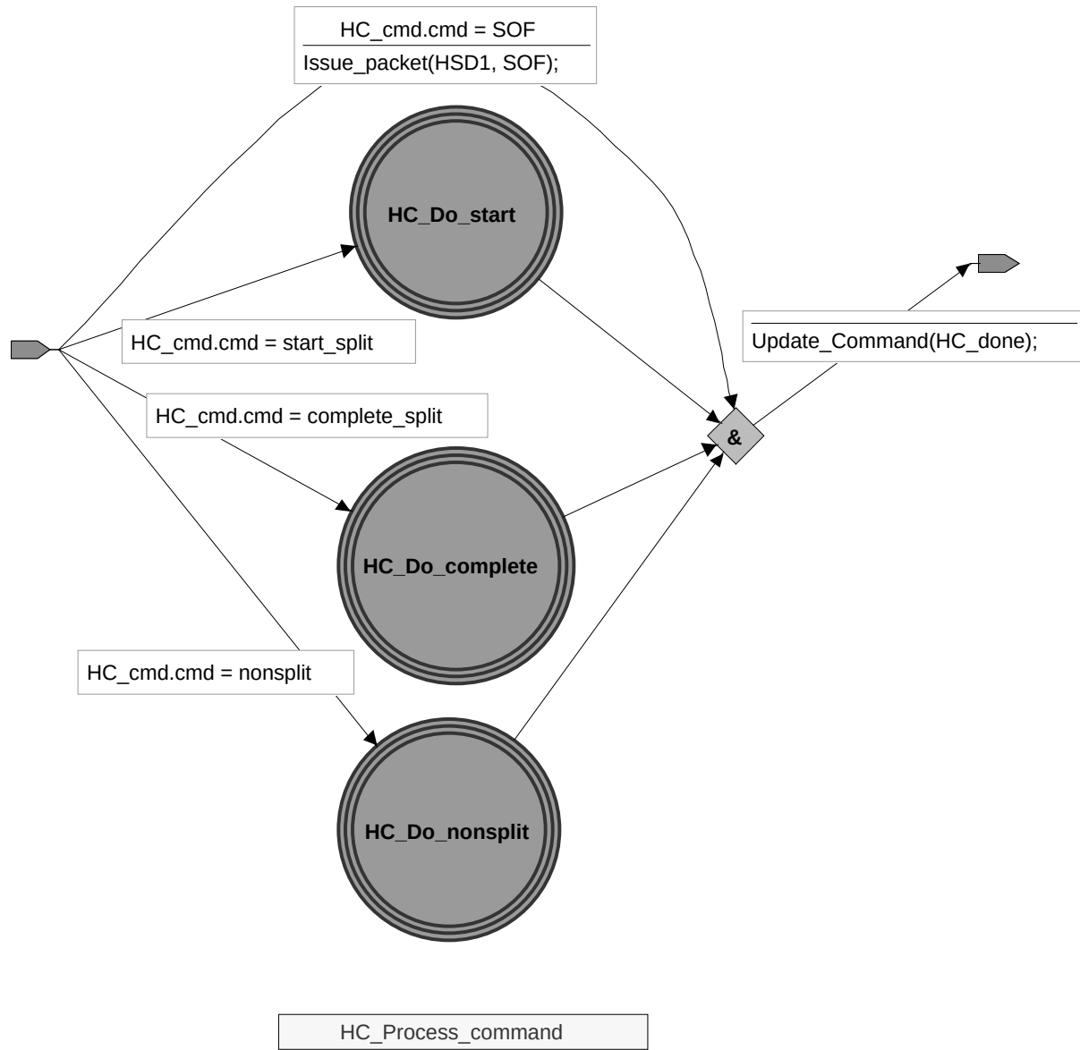
Figure 11-35. HC_Process_Command
