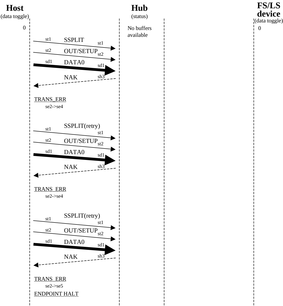
Figure A-17. No Buffer Available HS NAK(S) 3 Strikes Smash
