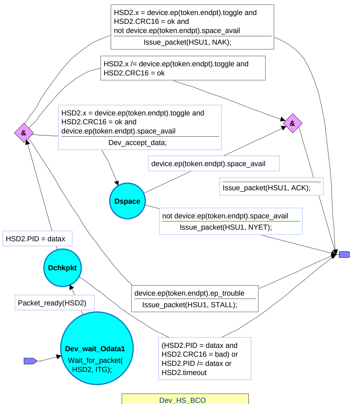
Figure 8-29. Device High-speed Bulk OUT /Control State Machine
