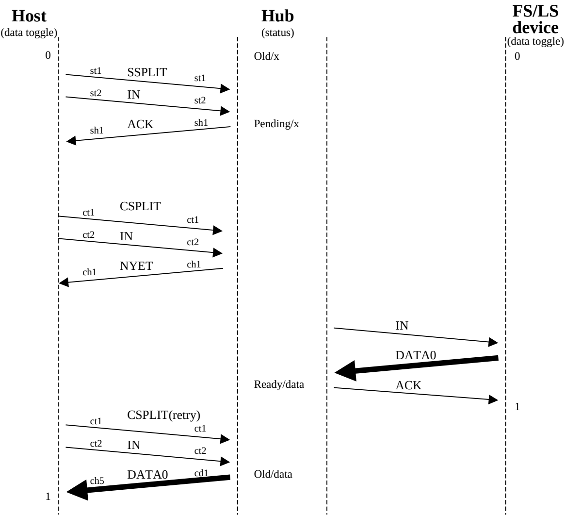
Figure A-42. CS Earlier No Smash(HS NYET)
