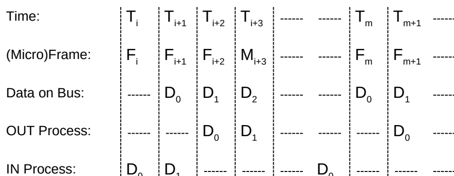
Figure 5-19. Data Prebuffering
