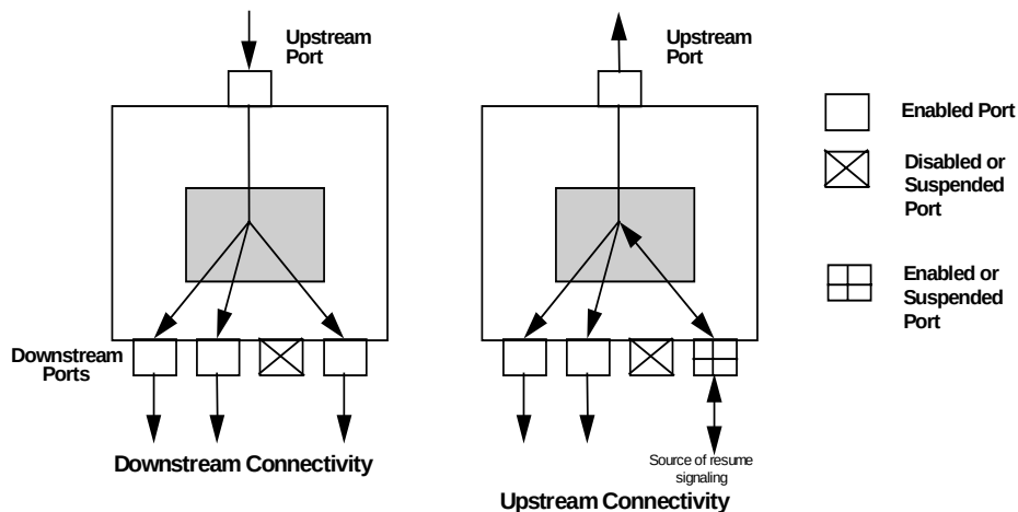
Figure 11-3. Resume Connectivity
