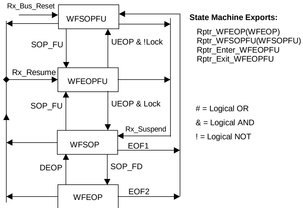
Figure 11-16. Hub Repeater State Machine
