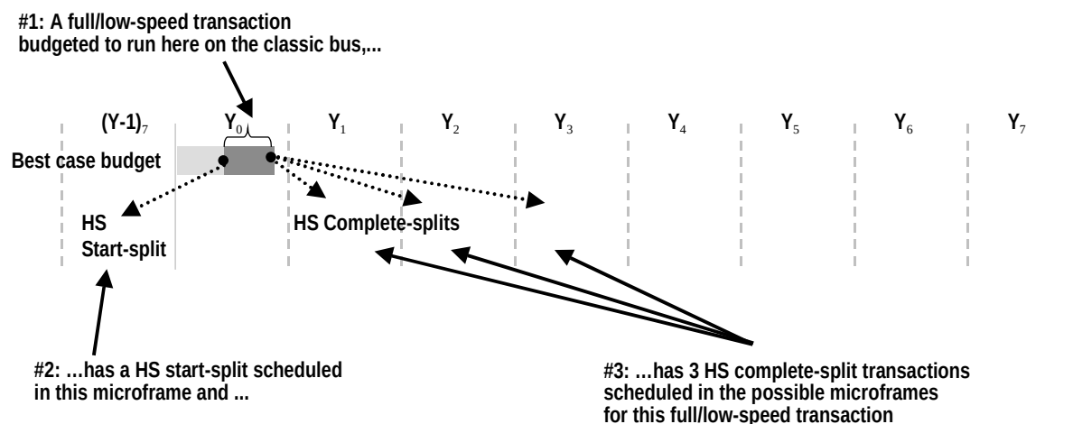
Figure 11-61. Scheduling of TT Microframe Pipeline
