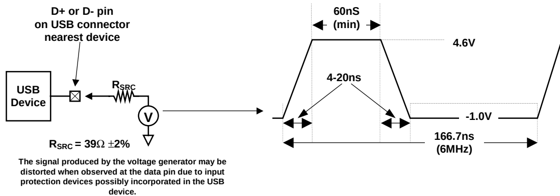
Figure 7-2. Maximum Input Waveforms for USB Signaling
