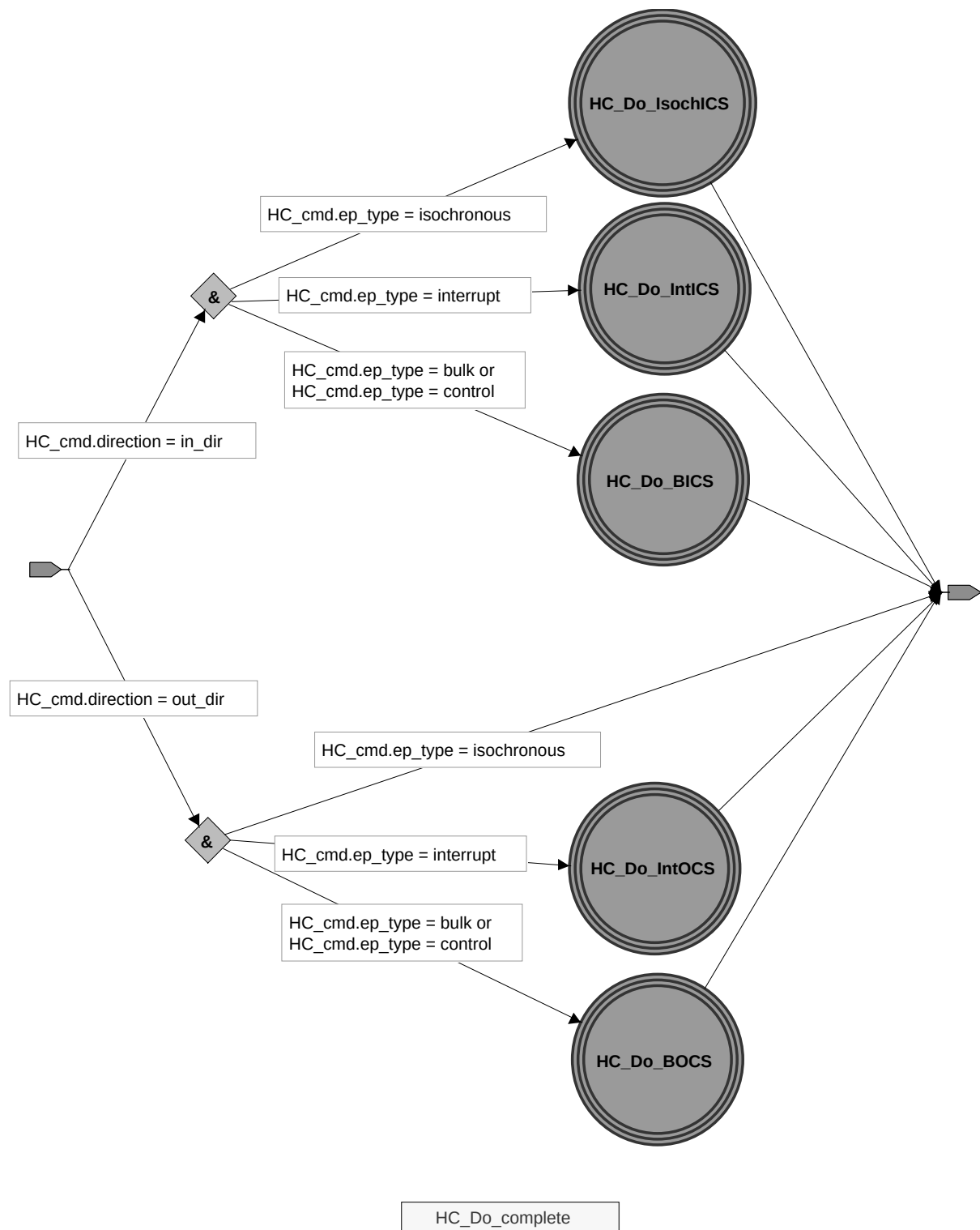
Figure 11-37. HC_Do_Complete
