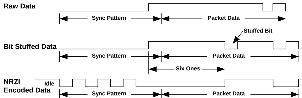
Figure 7-32. Bit Stuffing
