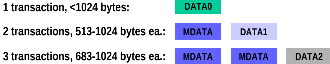
Figure 5-12. Data Phase PID Sequence for Isochronous OUT High Bandwidth Endpoints
