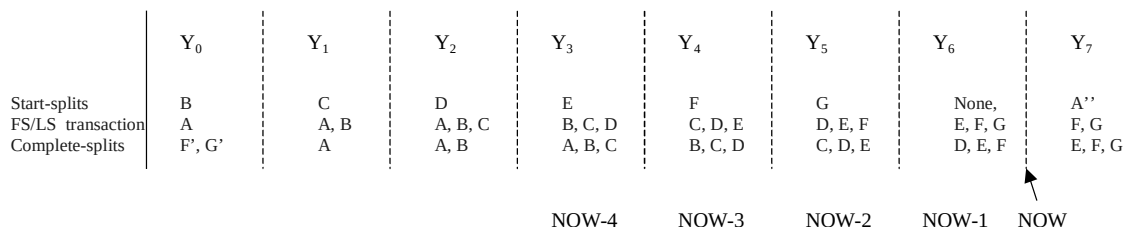
Figure 11-66. Microframe Pipeline
