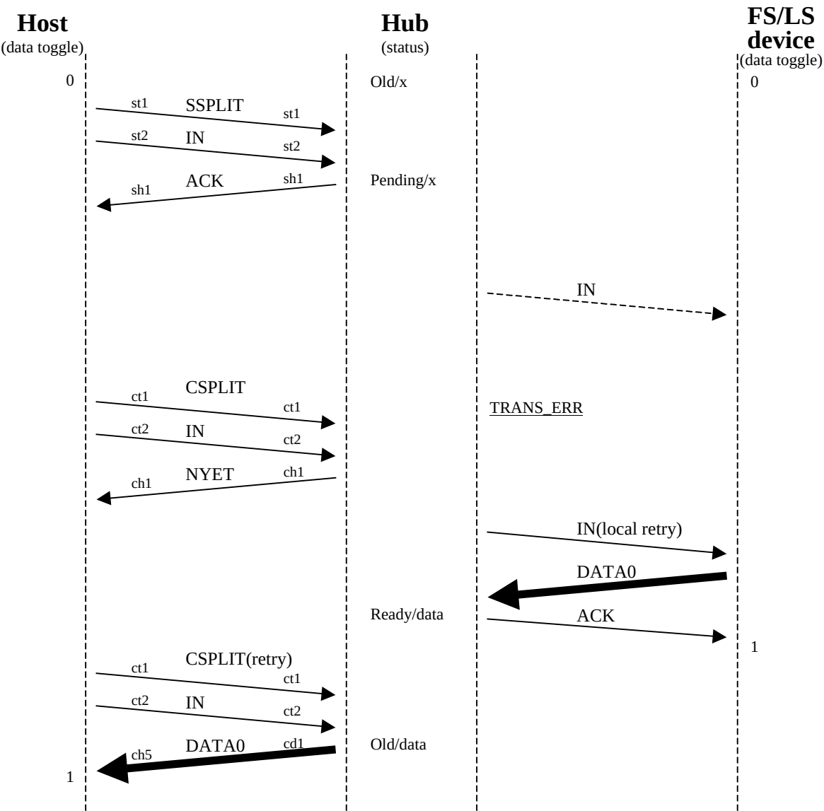
Figure A-34. Normal FS/LS IN Smash
