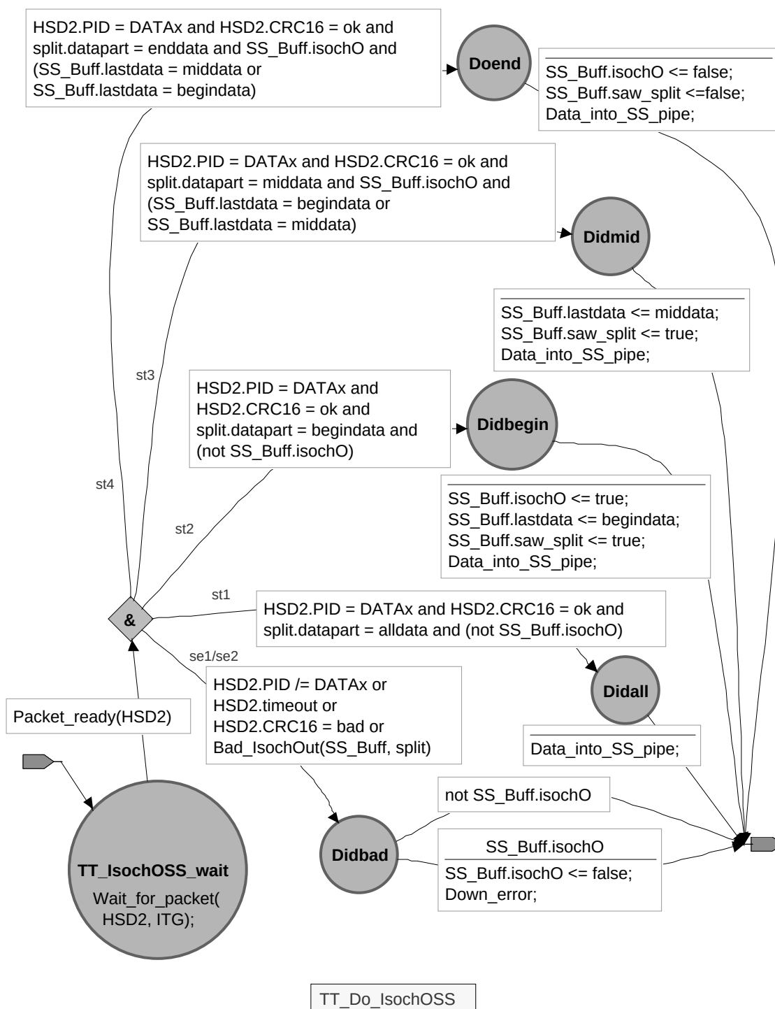
Figure 11-87. Isochronous OUT Start-split Transaction TT State Machine
