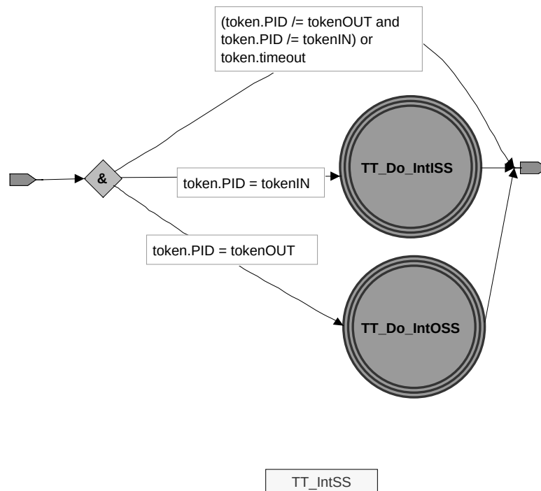
Figure 11-44. TT_IntSS
