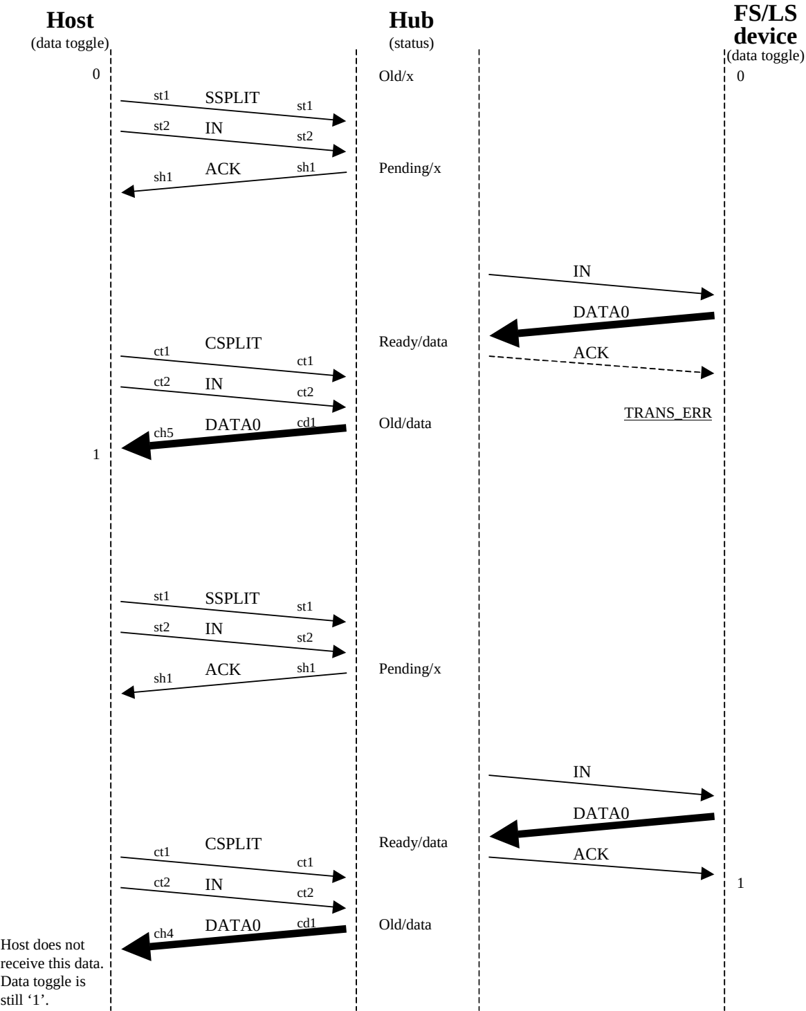
Figure A-38. Normal FS/LS ACK Smash
