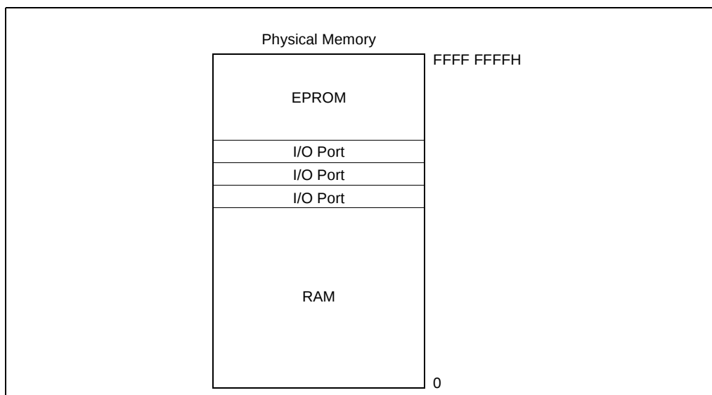
Figure 10-1. Memory-Mapped I/O
