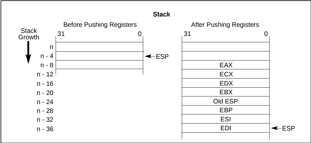
Figure 6-2. Operation of the PUSHA Instruction
